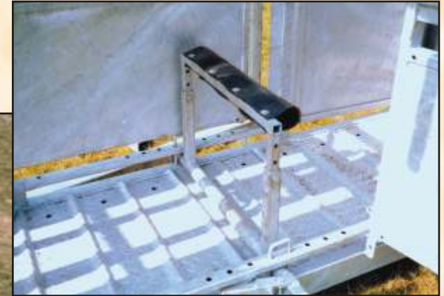
Anti-kick bar for belly trimming
